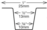
FRONT VIEW
